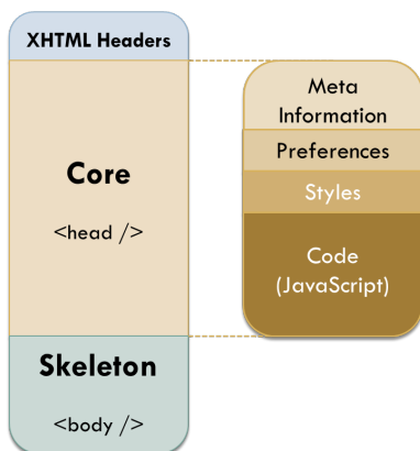
Figure 2. Schematic view representing the structure of the code for an UWA widget.
