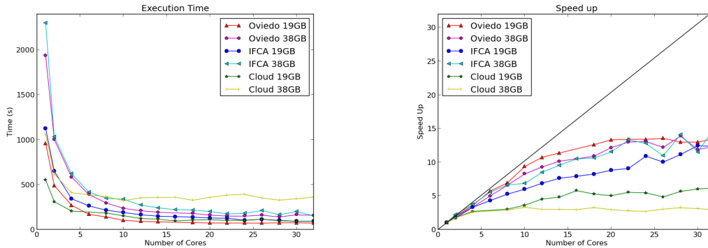
Figure 3. Time spent (left)= and speedup factor (right) using PAF over a different number of workers. Two samples of t\bar{t} MC events weighting 19 GB and a 38 GB were used. Three different PROOF modes are shown: PROOF Cluster (IFCA), PROOF Cloud (Cloud) and PoD (Oviedo). No significant gain is found above 20 nodes. This is thought to be due to the simplicity of the test and the high but limited bandwidth of the storage systems (GPFS at IFCA and HDFS at Oviedo)
