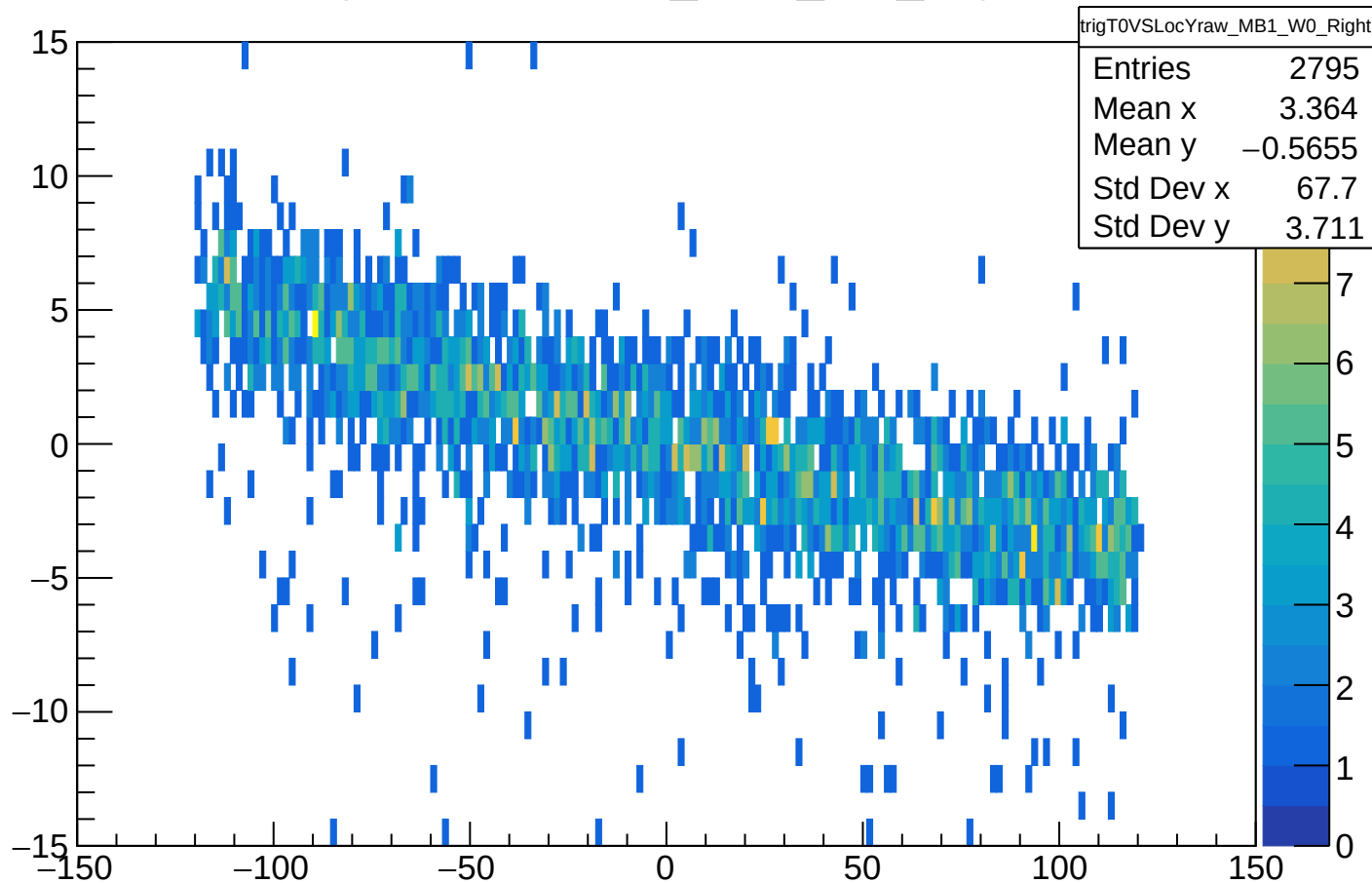
trigTOVSLocYraw_MB1_W0_Right
