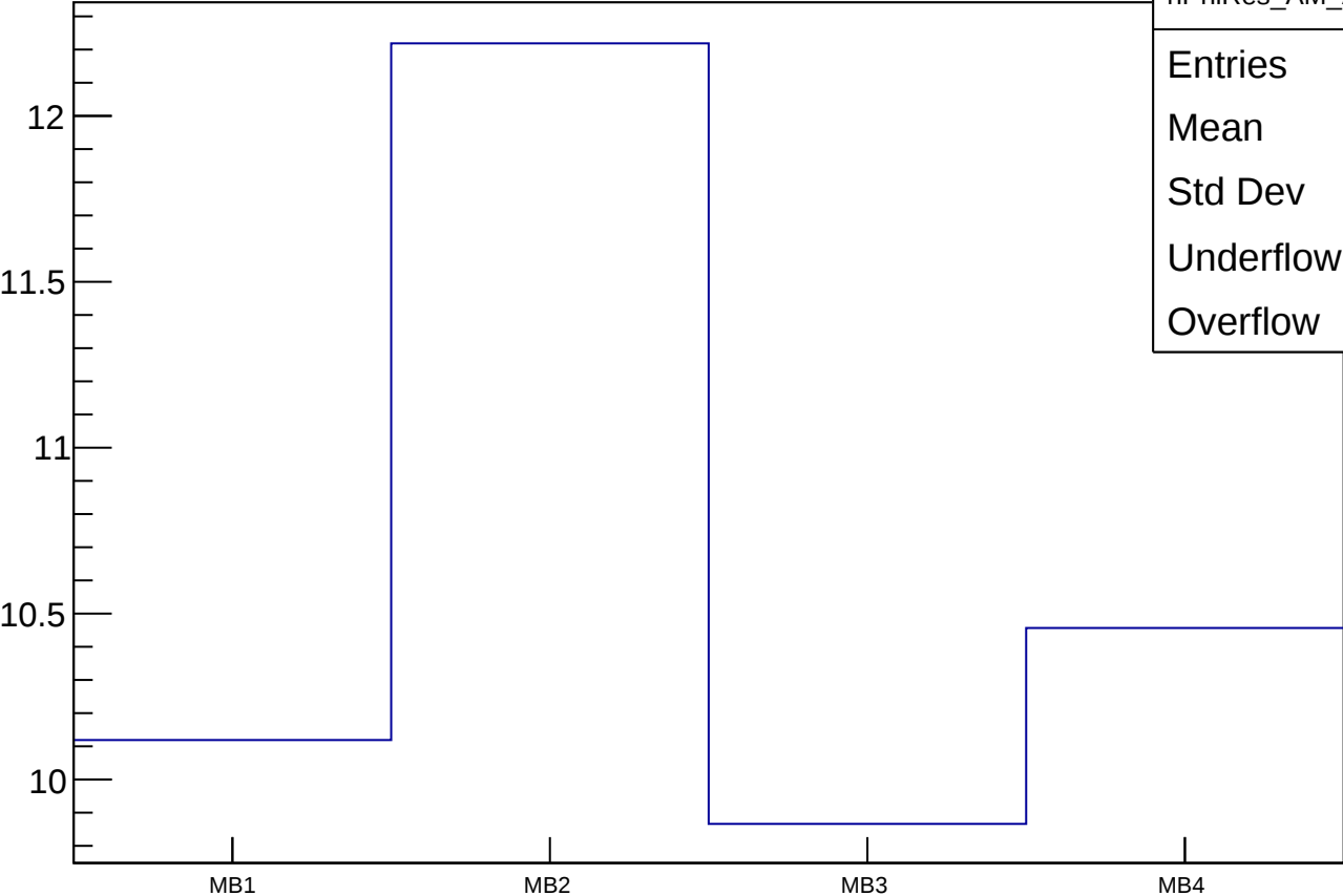
PhiRes Seg-TP distribution for Wh+1
