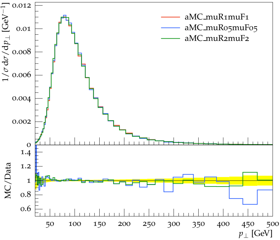
Transverse momentum distribution for jet 1
