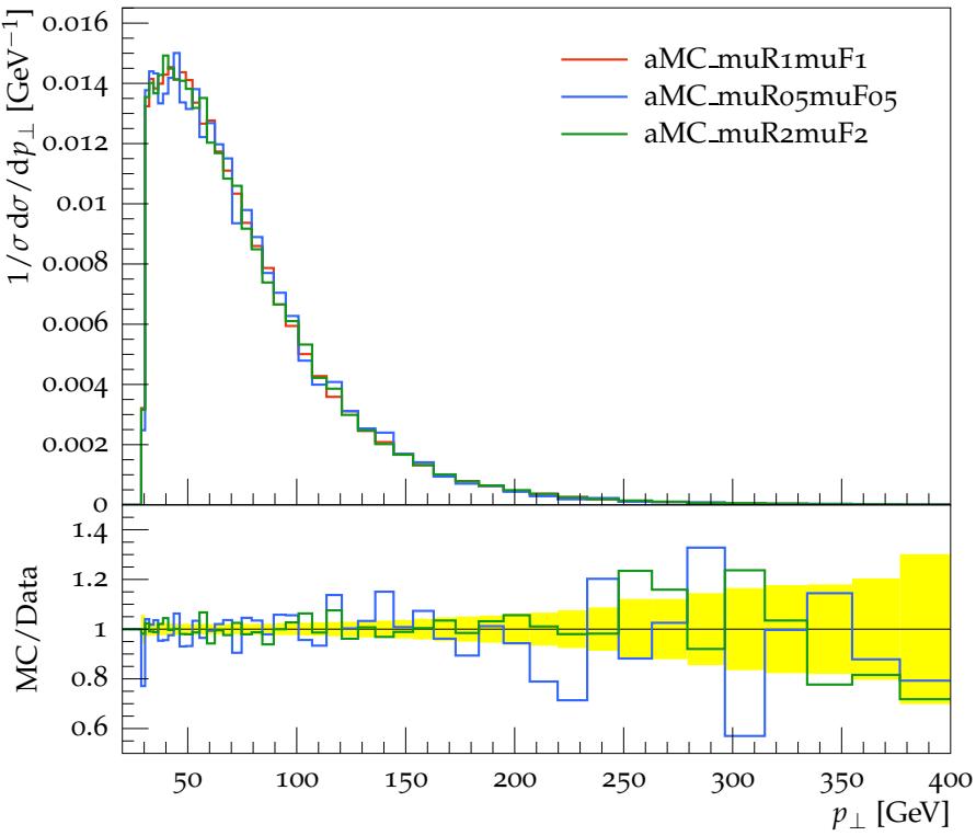
Transverse momentum distribution for b -jet 1
