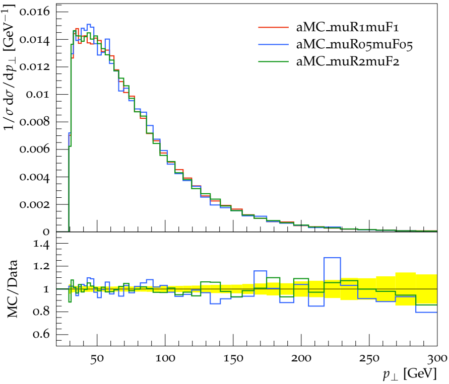
Transverse momentum distribution for b -jet 2
