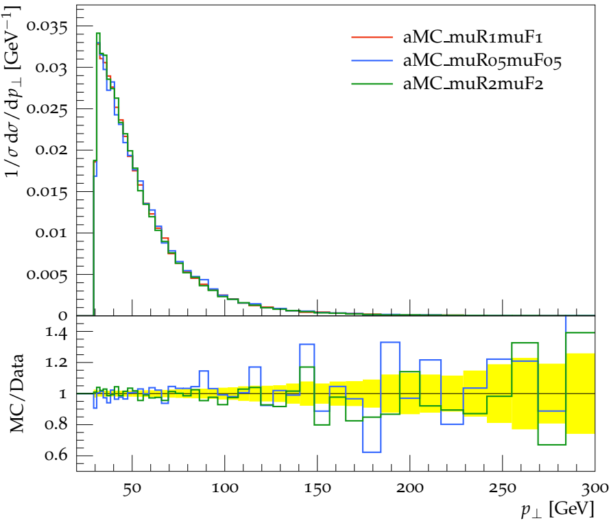
Transverse momentum distribution for light jet 2
