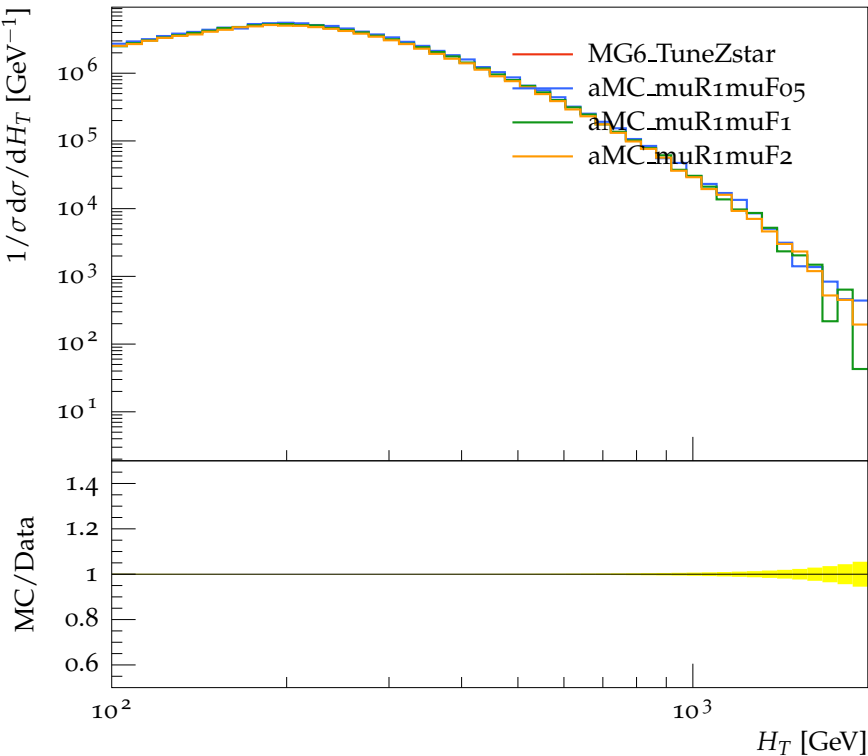
H_T distribution for all jets
