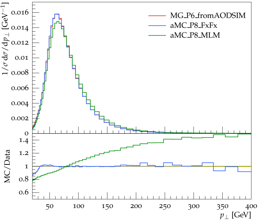
Transverse momentum distribution for jet 2
