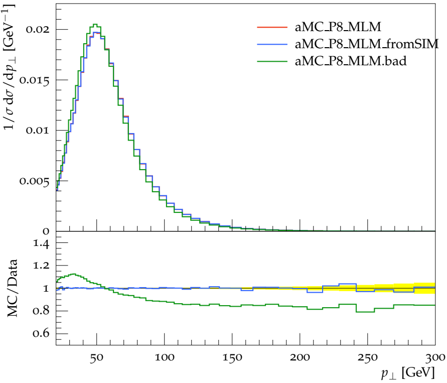
Transverse momentum distribution for jet 3
