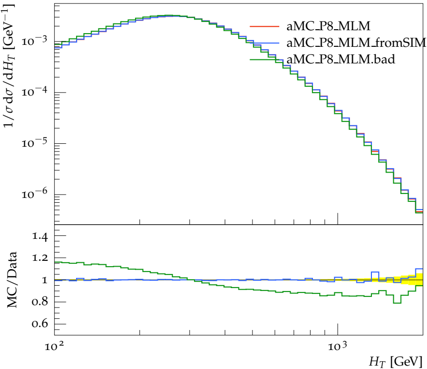
H_T distribution for all jets
