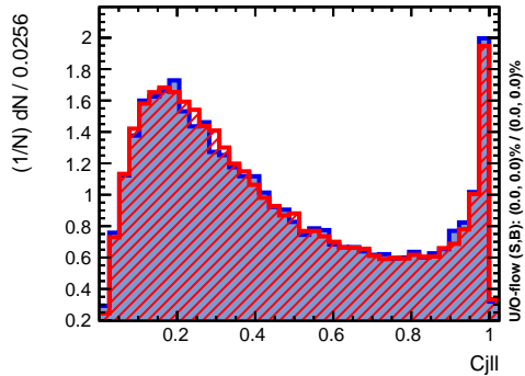
Input variable: Cjll
