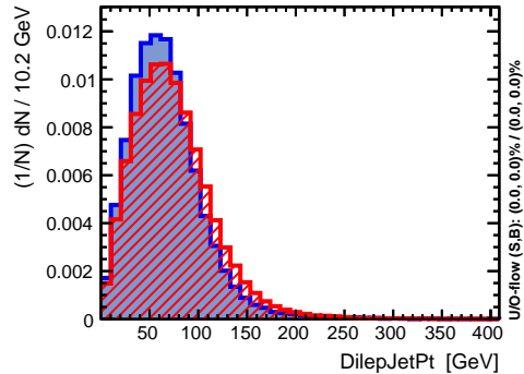
Input variable: DilepJetPt
